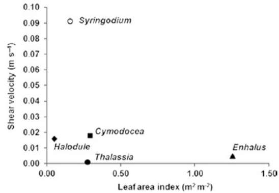
Figure 3: Shear velocity U^* (m s -1 ) versus leaf area index (m 2 m -2 ). U^* scales with shear stress, the force resulting from the vertical velocity gradient. The leaf area index, a common predictor of U^* , is the one-sided area of leaves per m 2 of substratum.
